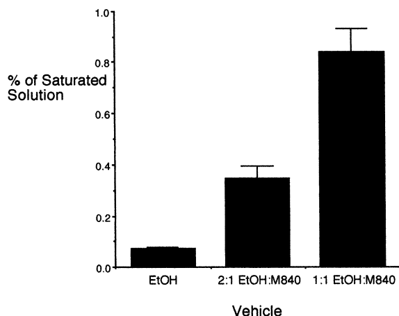
Fig. 6. Percentage of applied dose of doxycycline permeated across full-thickness human skin from three vehicles after 48 h.
