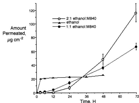
Fig. 2. Permeation of doxycycline across full-thickness excised human skin from ethanol, 1:1 and 2:1 ethanol/M840.
