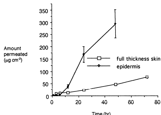
Fig. 3. Permeation of doxycycline 1:1 ethanol/M840 across heat-separated epidermis and full-thickness skin.
