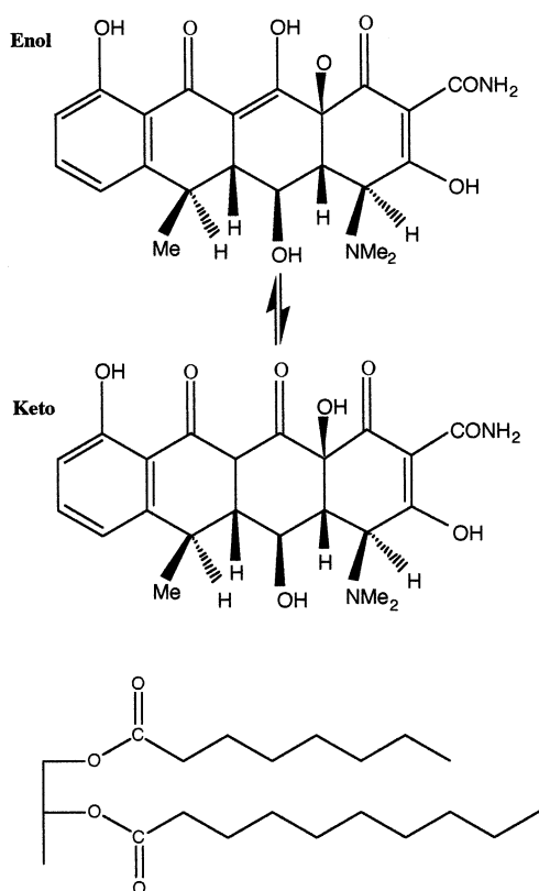
Fig. 1. Chemical structure of doxycycline tautomers and representative structure of Migliol 840.
