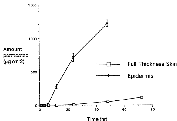
Fig. 4. Permeation of doxycycline 2:1 ethanol/M840 across heat-separated epidermis and full-thickness skin.
