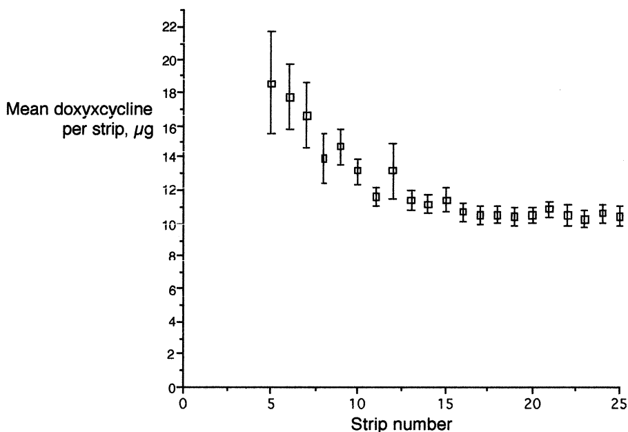
Fig. 5. Depth profile of doxycycline within heat separated epidermal membranes from 1:1 ethanol:M840 ( n = 5 , \pm SE).
